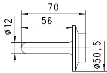
Sensor for Tri-clamp connection Type ..056..
