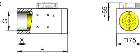
DN 50
