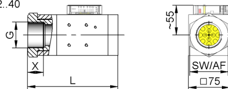
DN 32..40
