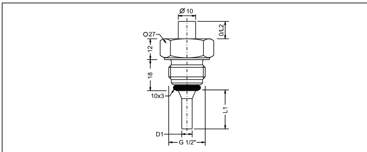
Type 4 / type 5 – Thread ISO 228-1 – G \frac{1}{2} "B, front-flush gasket
