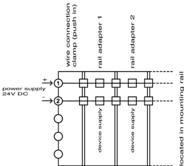
Figure 4 Terminal Assignment PRVK
