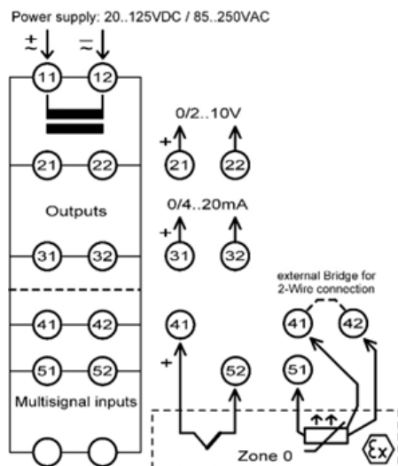
Figure 6 Connection Diagram
