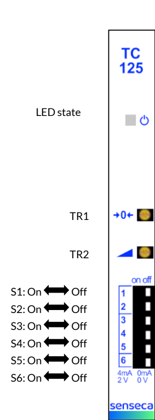
Figure 7 Control Elements
