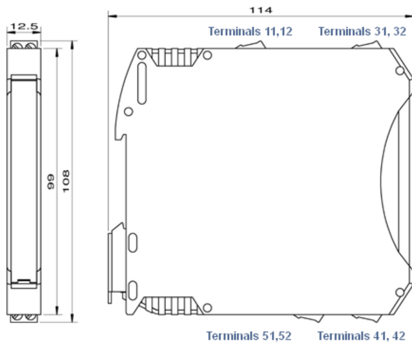
Figure 8 Dimensions
