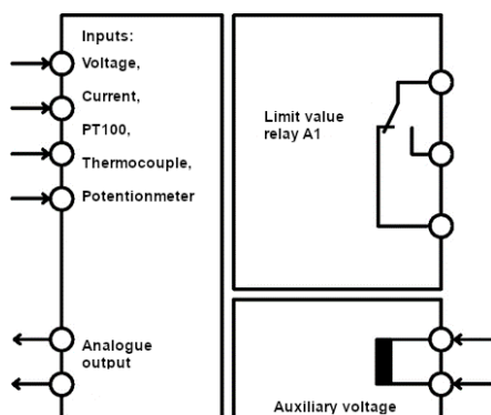
Figure 2 Block circuit diagrams
