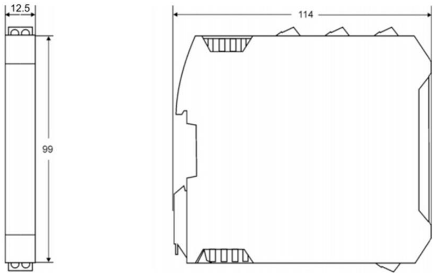
Figure 13 Dimensions
