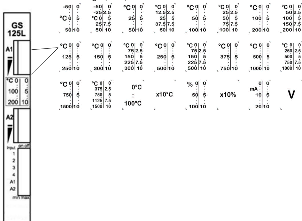
Figure 9 Scale marking
