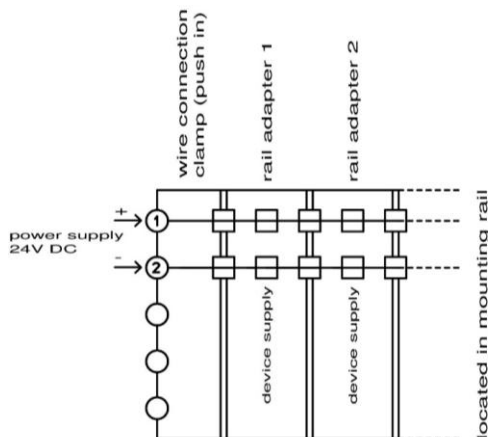
Figure 5 Terminal Assignment PRVK
