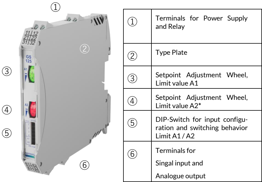
Figure 1 Limit switch GS125
