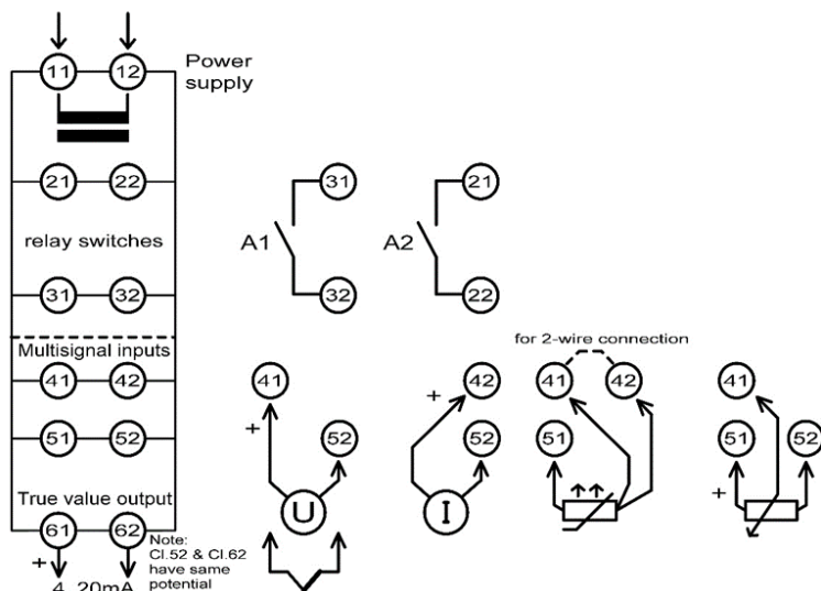
Figure 8 Connection Diagram GS125x-3
