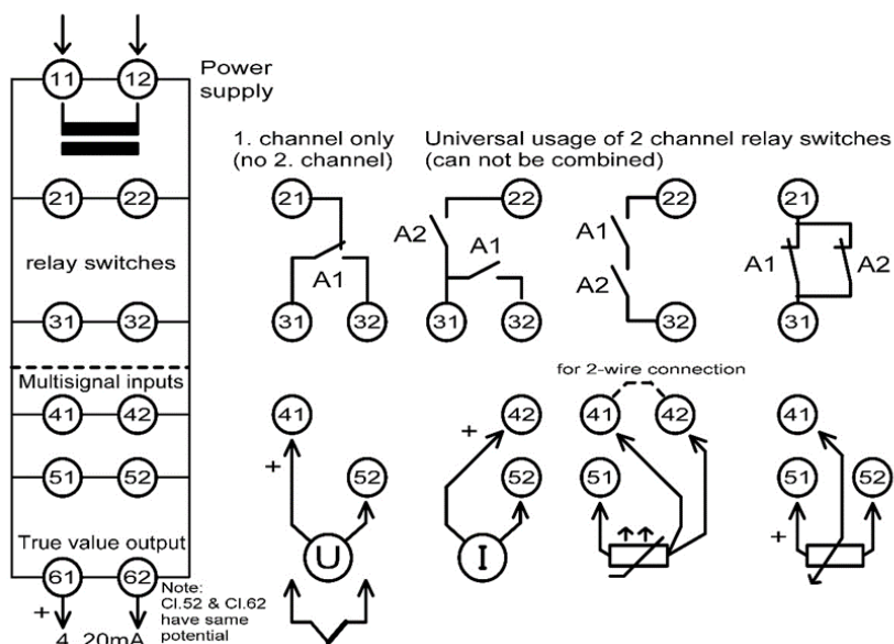
Figure 7 Connection diagram GS125x-1, GS125x-2
