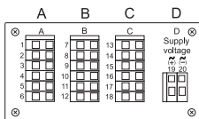
Terminal strip position
