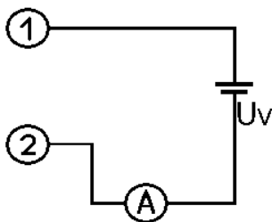
2-wire connection (4-20mA)
