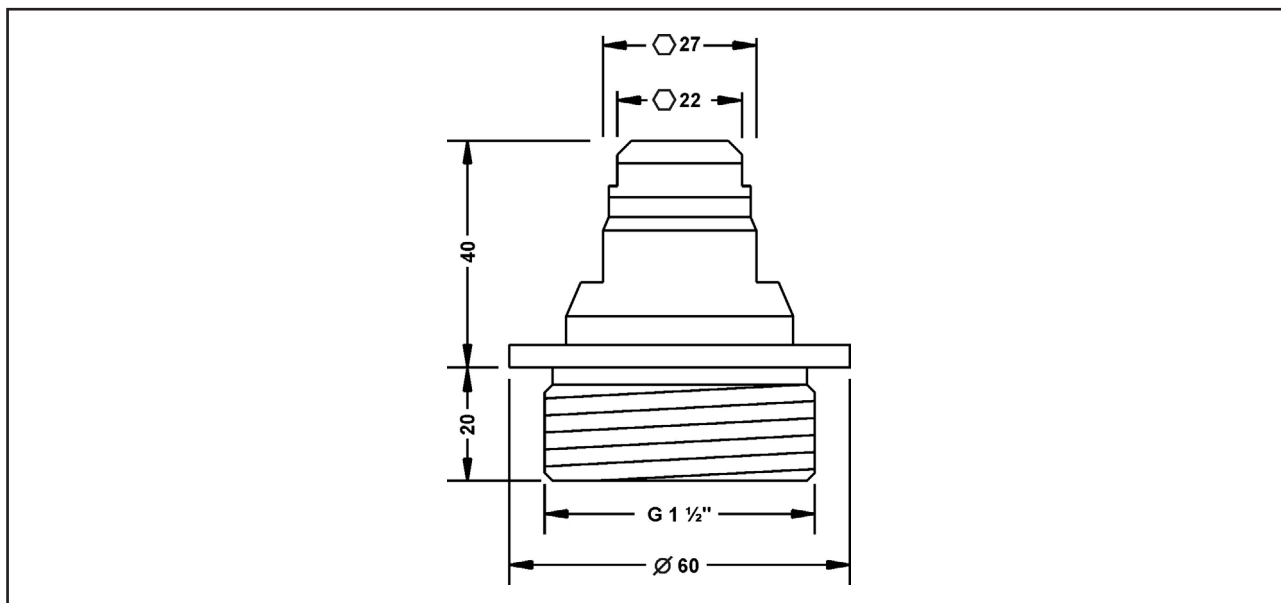
Accessory screw plug G 1½" ISO 228-1, for cable Ø10mm
