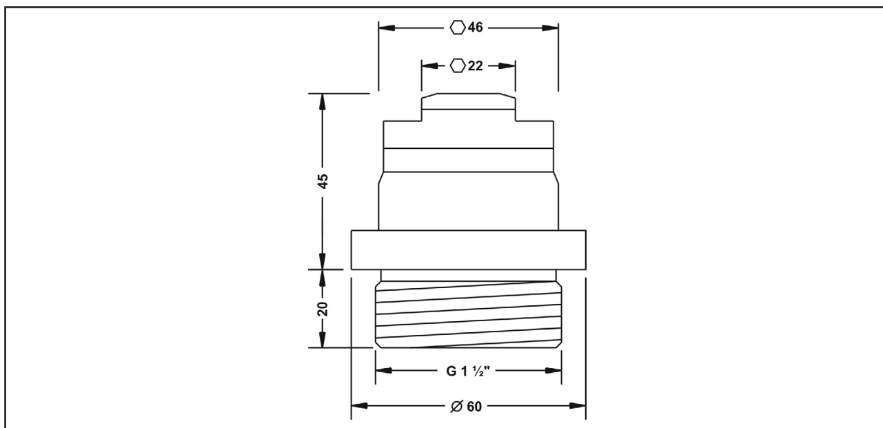
Accessory screw plug G 1½" ISO 228-1, PEEK, for cable Ø10mm
