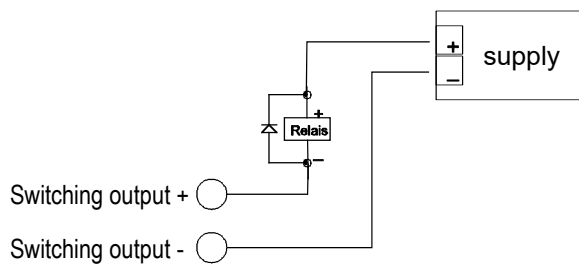
Assignment as low-side switch
