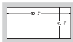
Panel cut-out
