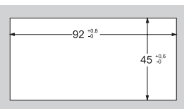
Panel cut-out
