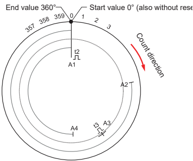
Example ring counter
