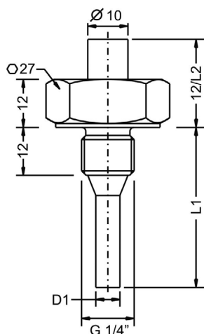
Type 3 – Thread ISO 228-1 – G 1/4" B
