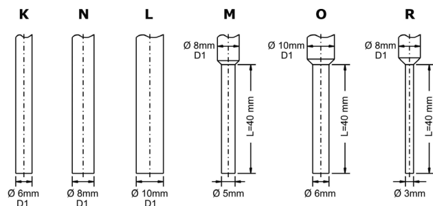
Sensor tube
