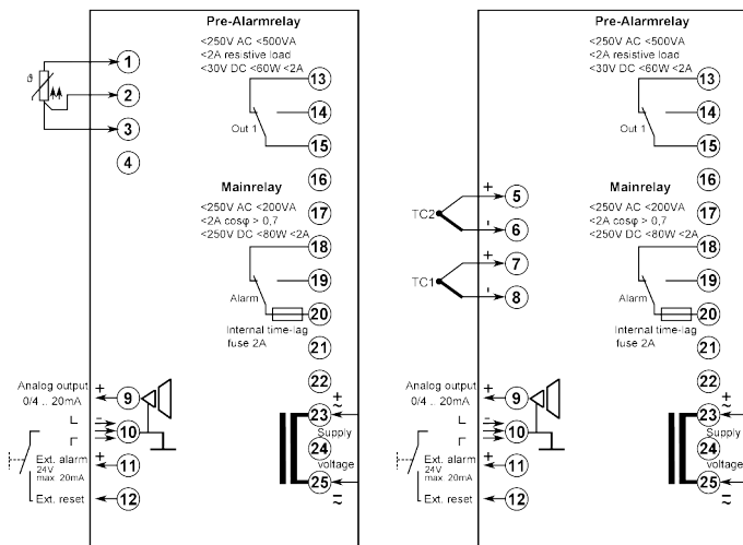
Pt100-2RQO
