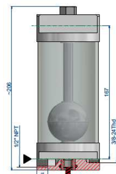
Type NG1..2
