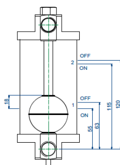
Type NG1..2
