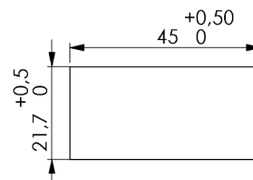
Panel cut-out
