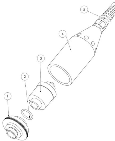
GOO housing
