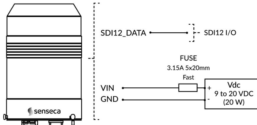
Fig. 3.4: Connections – SDI12
