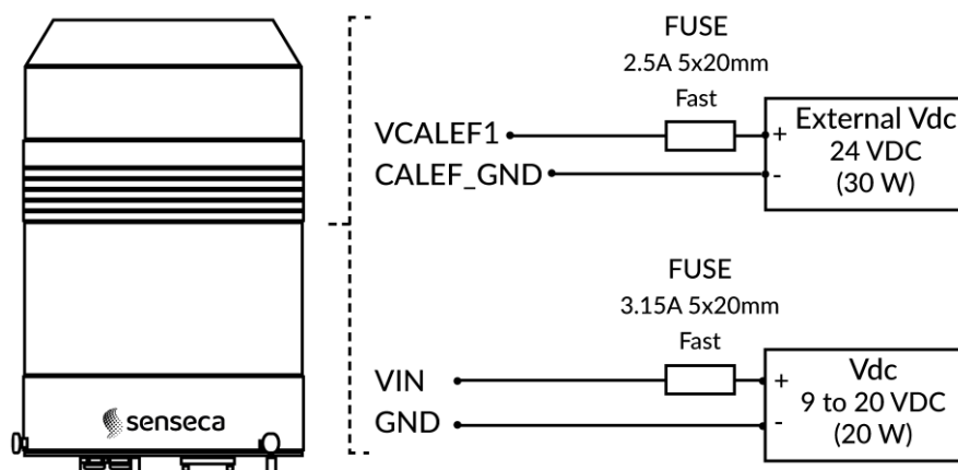
Fig. 3.5: Connections - Heater
