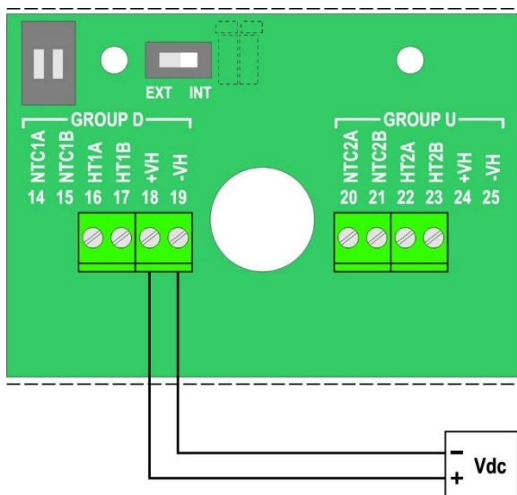
Modelli RTD...Fx, RTD...Dx e RTD...Vx Morsetti a vite
