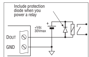
Typical connection for alarm relay activation
