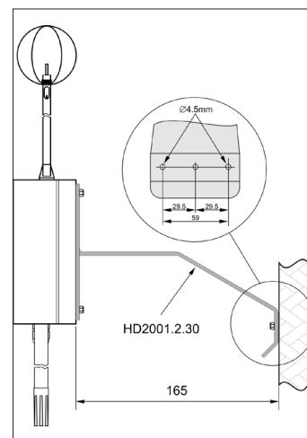
Support for model HD2001.2
