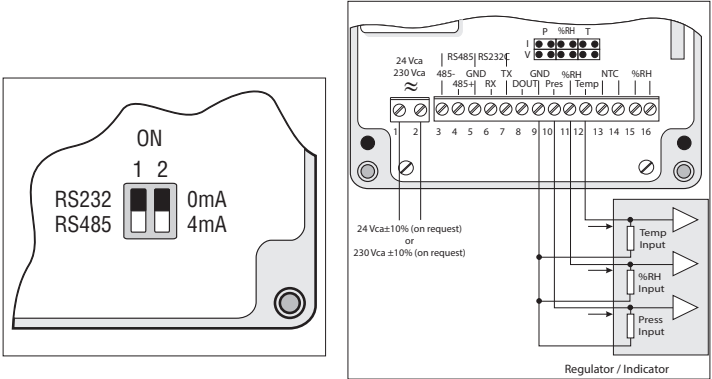
Selection dip switch for protocol RS232/RS485 and analogue output.
