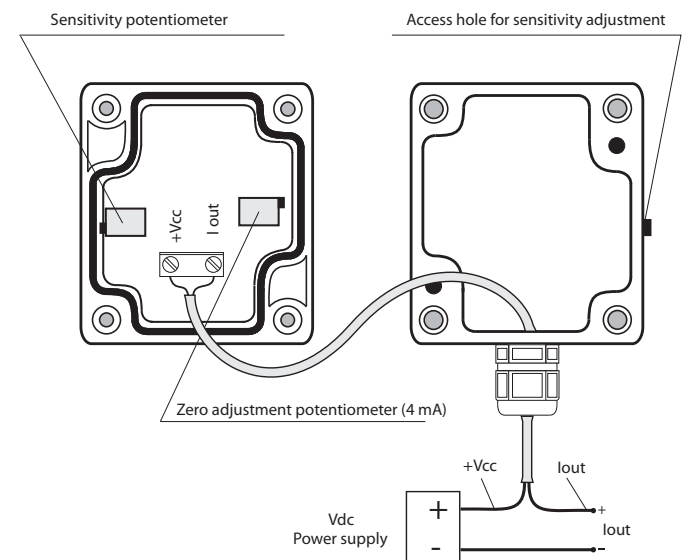
Fig. 2 - Connecting diagram with current output
