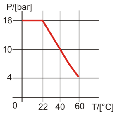
Temperature-pressure diagram PVC-U
